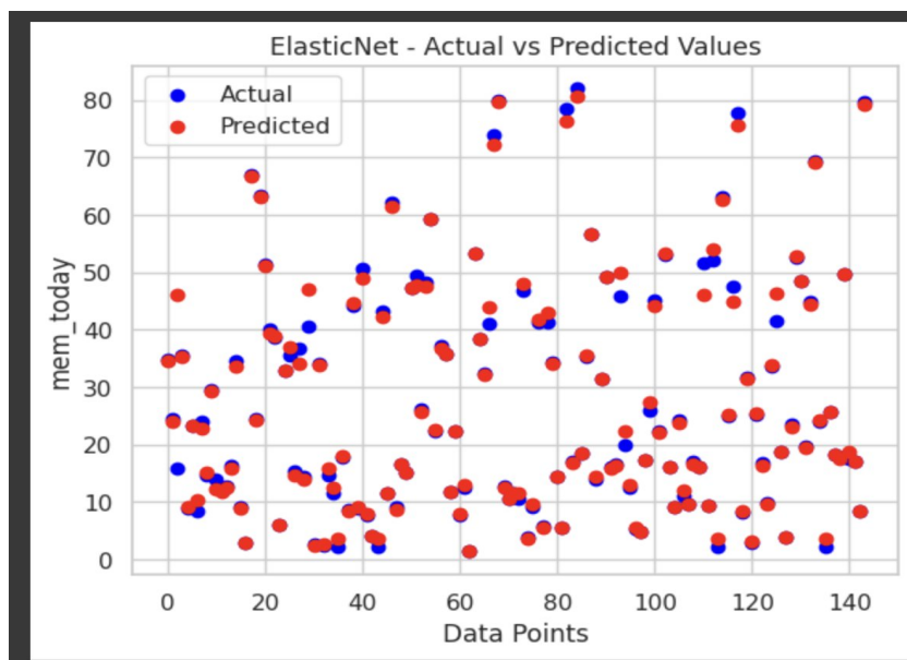
Figure 11. The graph with actual and predicted(via ElasticNet) memory usage.
